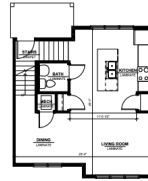
2 Main Level Floor Plan SCALE: 1/4" = 1'-0"
