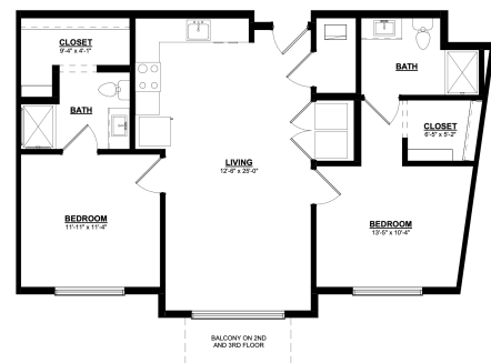
DISTRICT PLACE | UNIT PLAN -x08 08 / 28 / 2023
